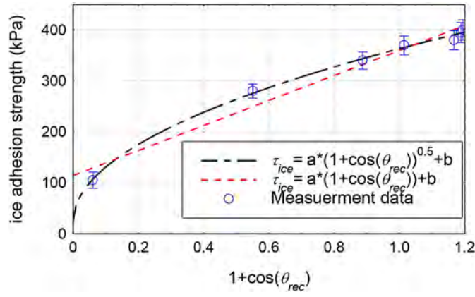
Fig. 11. Measured ice adhesion strength on the SHS coated test plate at T_{surface} = -10^{\circ}\text{C} against the contact angle scaling parameter of [1 + \cos \theta_{rec}] .
