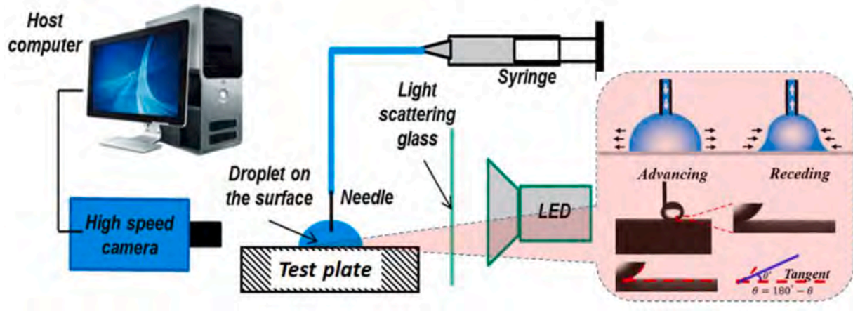
Fig. 4. The experimental setup to measure contact angles of droplets on the test surfaces.
