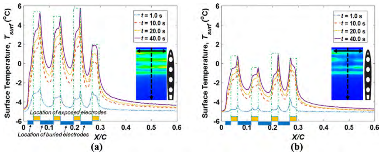
Fig. 7. The spanwise-averaged temperature profiles along the airfoil chord with the plasma actuators being operated at the power of P = 40 W, under a dry test condition of U_{\infty} = 40 m/s, T_{\infty} = -5^{\circ}\text{C} and LWC = 0 g/m 3 . (a) Plasma actuation in the duty-cycled mode ( f_{\text{duty-cycle}} = 1 Hz) at V_{p-p} = 14 kV, f = 10 kHz; (b) plasma actuation in the continuous mode at V_{p-p} = 11.5 kV, f = 10 kHz.
