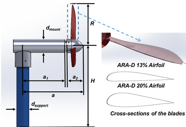
Fig. 1. Schematic of the UAS propeller model used in the present study.
